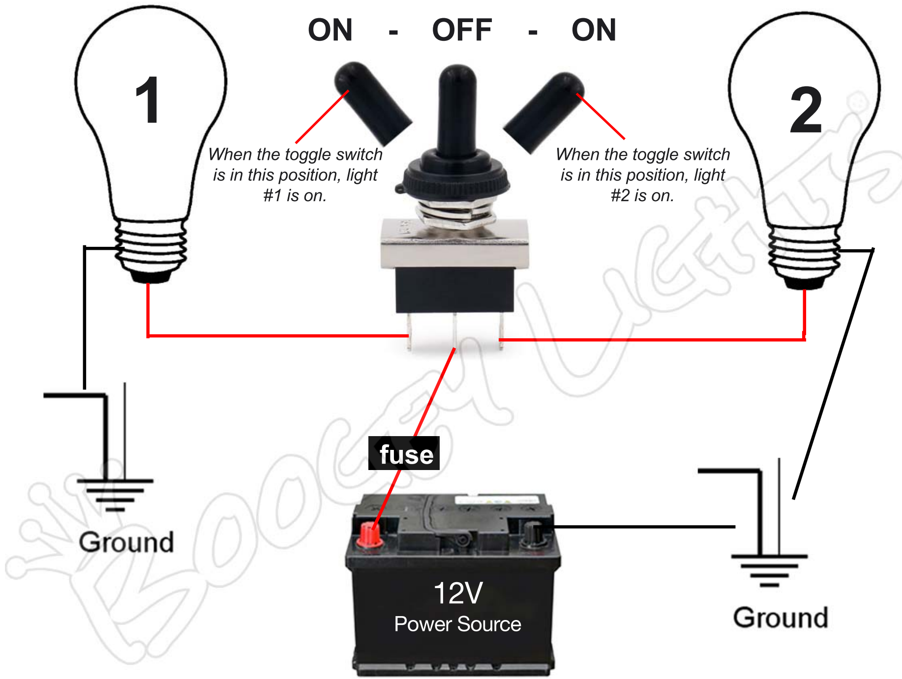
ON-OFF-ON toggle switch wiring diagram. Do not exceed switch AMPERAGE rating.
